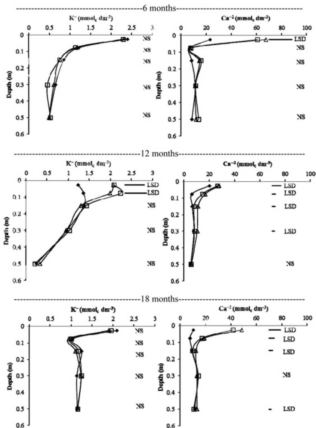
Figure 5. K^+ and Ca^{2+} levels after 6, 12 and 18 months from the application of lime (□), silicate (Δ) and the control (●). Vertical bars indicate the least significant difference (LSD)
