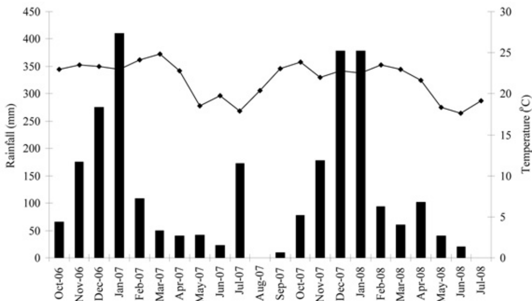
Figure 1. Temperature and rainfall during the study period, from October 2006 to July 2008
