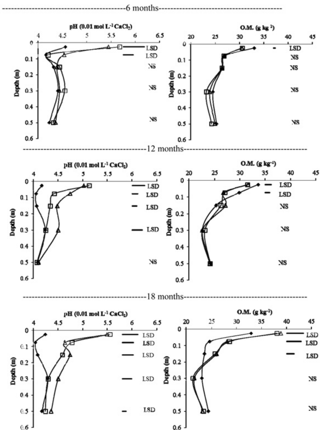
Figure 2. pH and organic matter (O.M.) level after 6, 12 and 18 months from the application of lime (□), silicate (Δ) and the control (▲). Vertical bars indicate the least significant difference (LSD)
