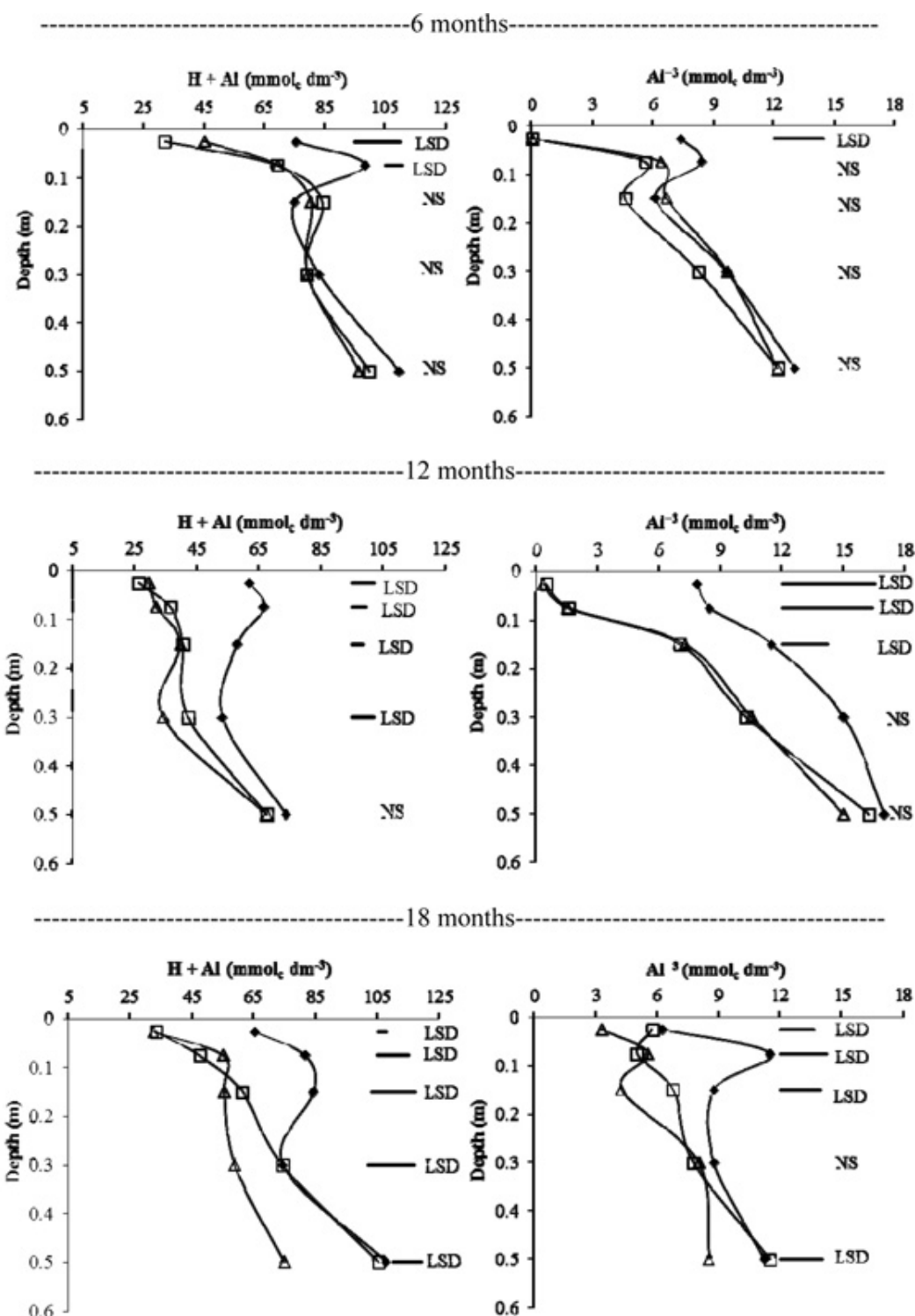
Figure 3. H + Al and Al 3+ levels after 6, 12 and 18 months from the application of lime (□), silicate (Δ) and the control (▲). Vertical bars indicate the least significant difference (LSD)
