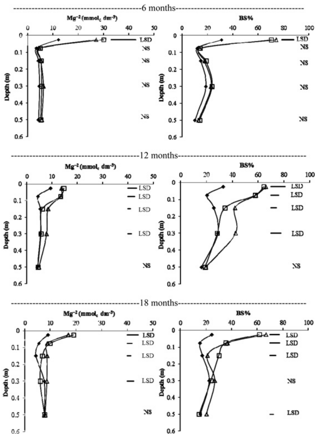
Figure 6. Mg^{2+} and Base Saturation (BS) levels after 6, 12 and 18 months from the application of lime (□), silicate (Δ) and the control (▲). Vertical bars indicate the least significant difference (LSD)
