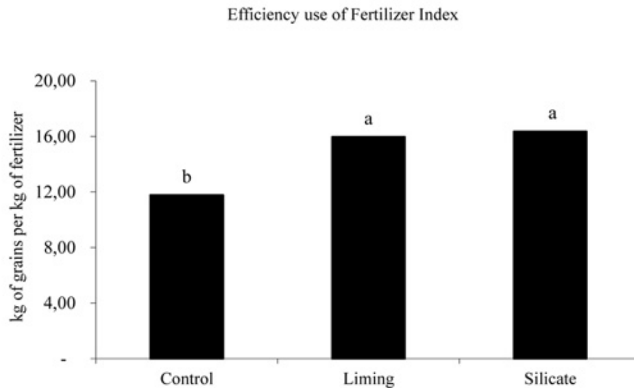
Figure 7. Efficiency use of fertilizers applied on soybean and maize affected by surface liming and silicate application under no tillage system. Columns followed by different letters differ statistically by the t test ( p < 0.05 )
