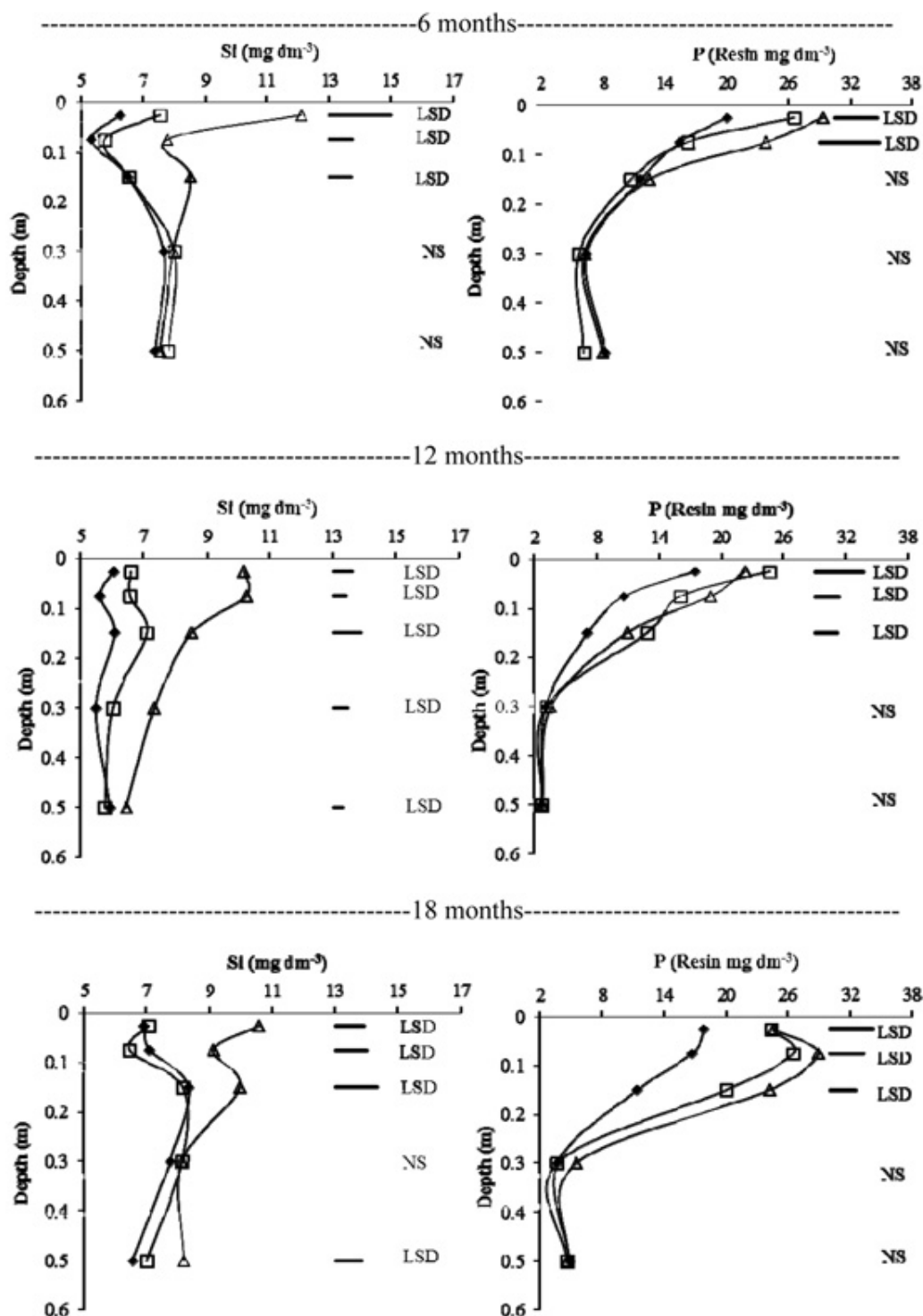
Figure 4. Si and P resin levels after 6, 12 and 18 months from the application of lime (□), silicate (Δ) and the control (▲). Vertical bars indicate the least significant difference (LSD)
